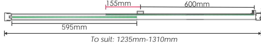
EDEN-T1220 (P-Silver) & EDEN T-1220B (Black)
