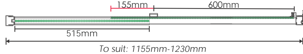
EDEN-T1140 (P-Silver) & EDEN T-1140B (Black)
