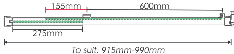
EDEN-T980 (P-Silver) & EDEN T-980B (Black)
