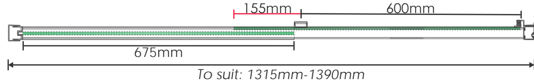
EDEN-T1300 (P-Silver) & EDEN T-1300B (Black)
